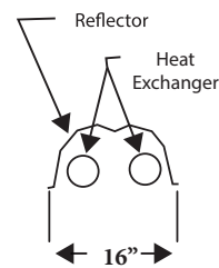
-End View-
