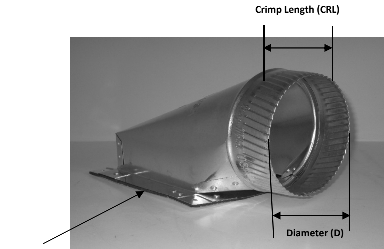
Flange (FLG)
